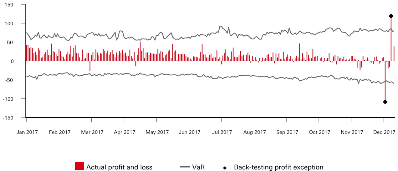
VaR back-testing exceptions against hypothetical profit & loss ($m)
